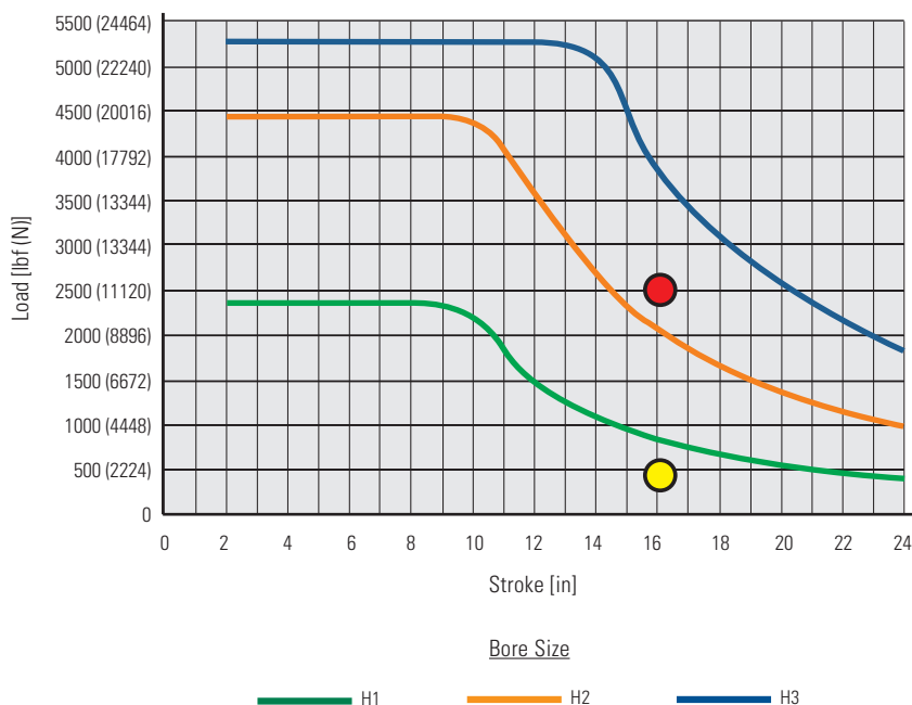
Stroke vs. Load and Bore Size
